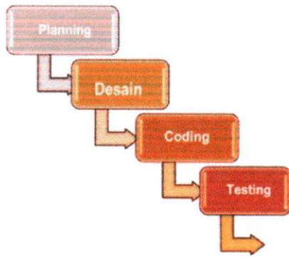
Figure 1 XP Metode
